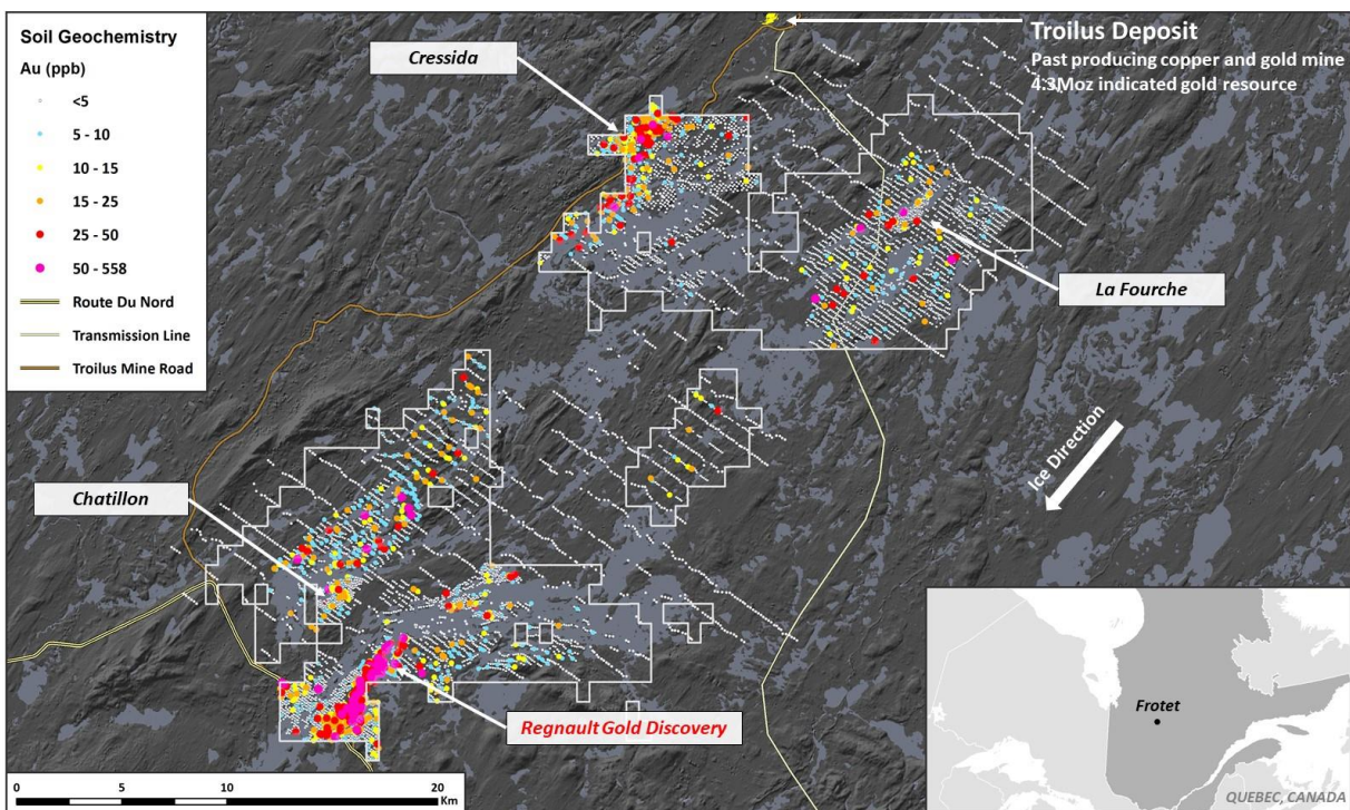
Figure 2. Map of Frotet Project showing Regional Till Sampling Geochemical Results
