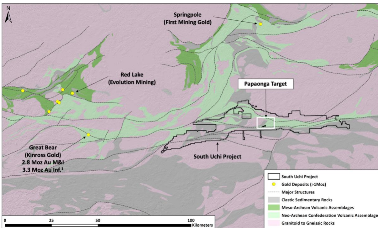
Figure 1. Regional volcanic assemblages with significant gold deposits and South Uchi Project location
