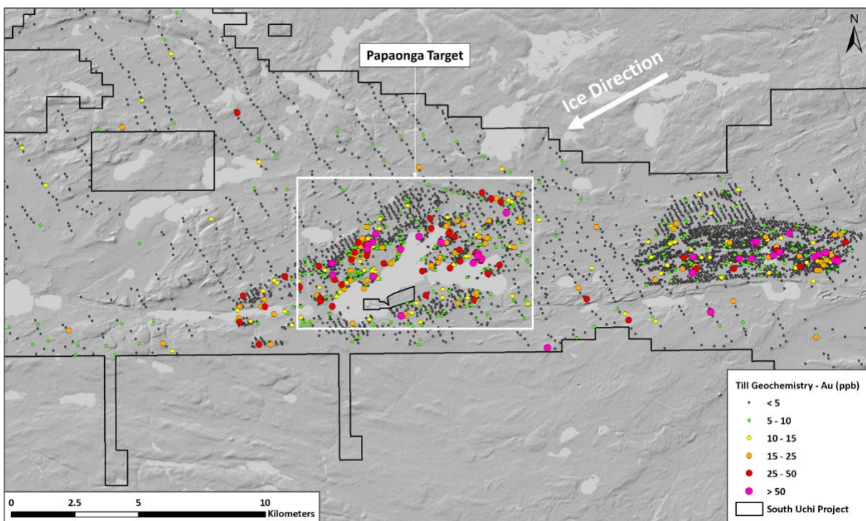
Figure 2. Map of Papaonga target area showing regional till sampling geochemical results
