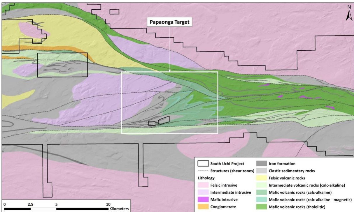
Figure 3. Geological map of Papaonga Target area
